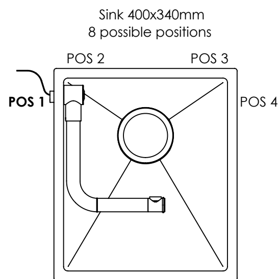
Mounting positions with Queensize Camper sinks
