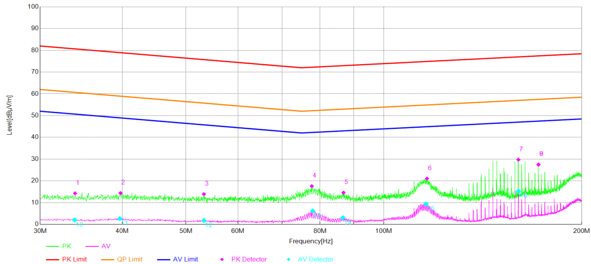
Vertical Polarity Test Result Diagram (Broadband and Narrow band)
